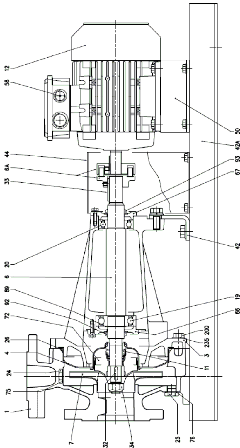
3DP4 SECTIONAL VIEW DRAWING
