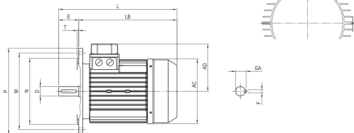
Dimensional sketch B5
