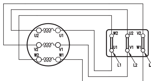
DELTA CONNECTION (Δ)
