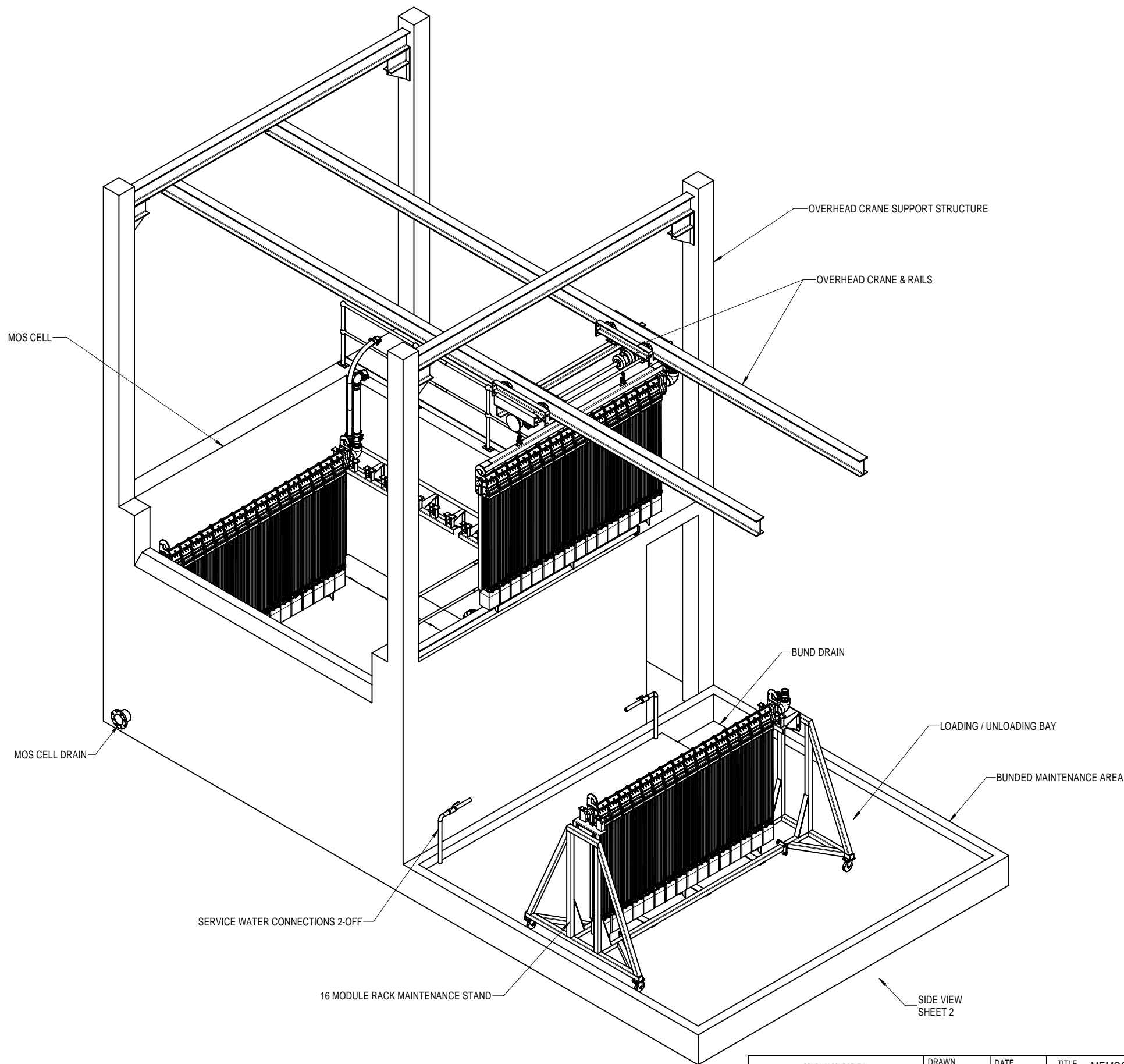
ISOMETRIC VIEW
